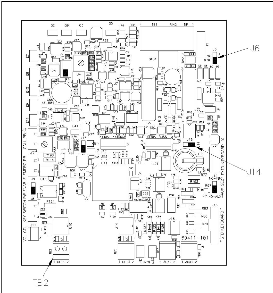
Figure 10. S.M.A.R.T. Phone PCBA
