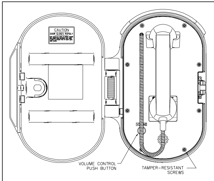
Figure 3. Model 227-003 S.M.A.R.T. Phone with spring loaded door in the open position
