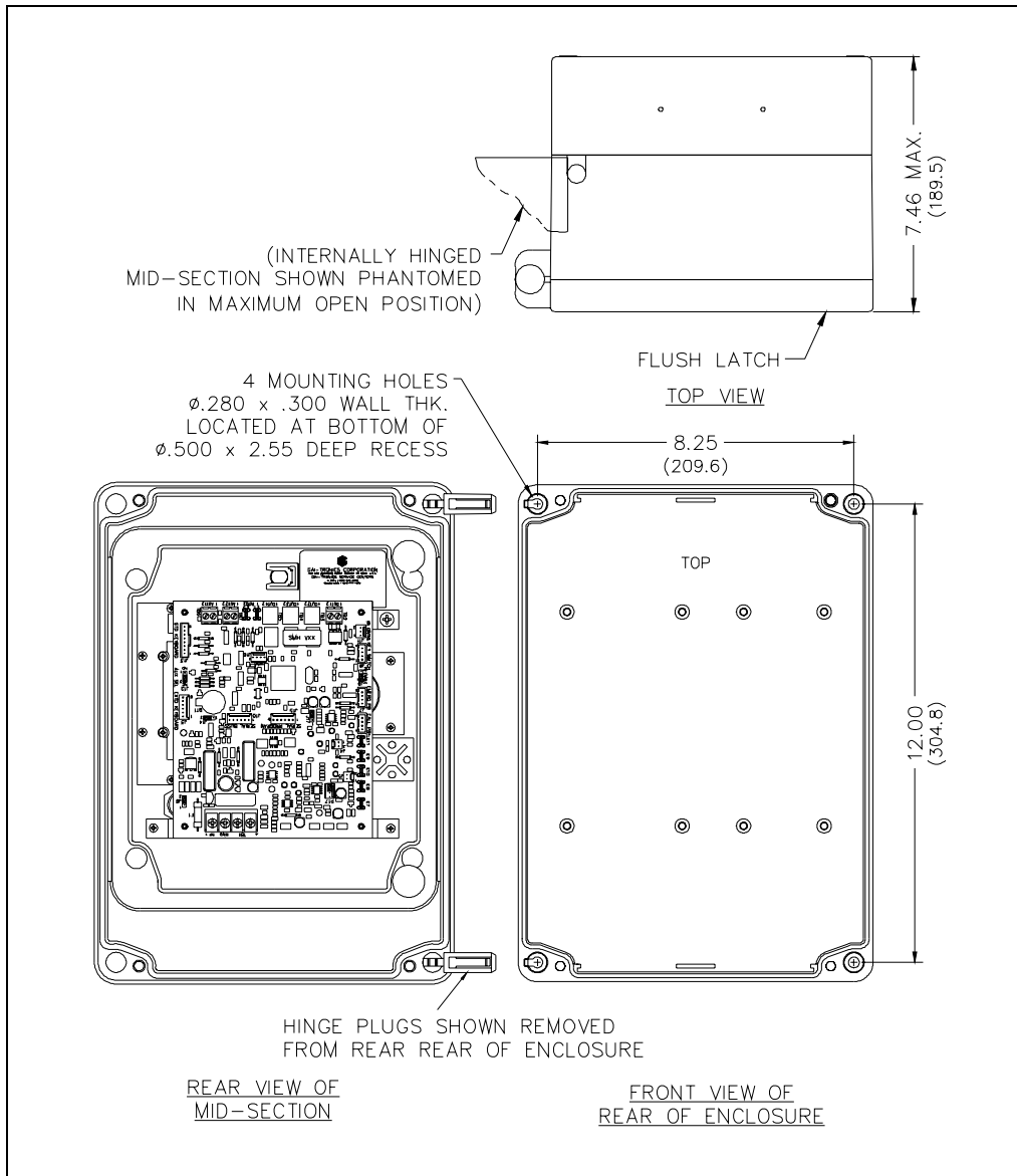
Figure 7. Model 257-003 Mounting Details
